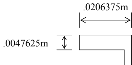
Figure 17. Microstrip Patch Antenna Dimensions
